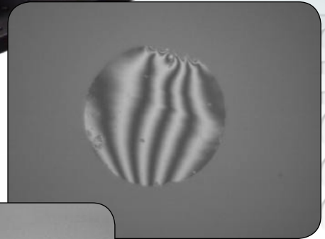
View fringes to check cleave angle
